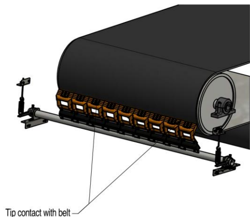
Fig. 3b Cleaner aligned with belt
